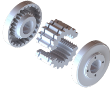
Coupling Kit
